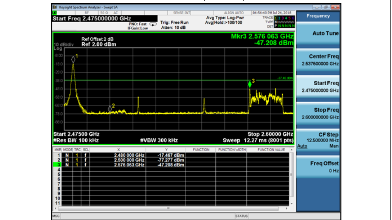
Mode 1 CH39 (2480MHz)
